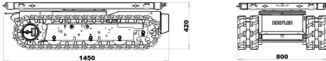
Figure 3: front and side view TC1
